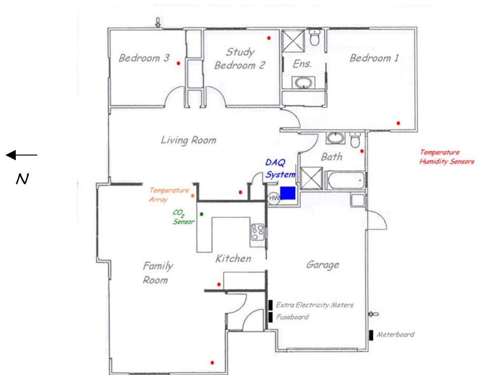
Figure 2 Floor plan of the Waitakere NOW Home® (North is to the left) showing monitoring equipment locations
