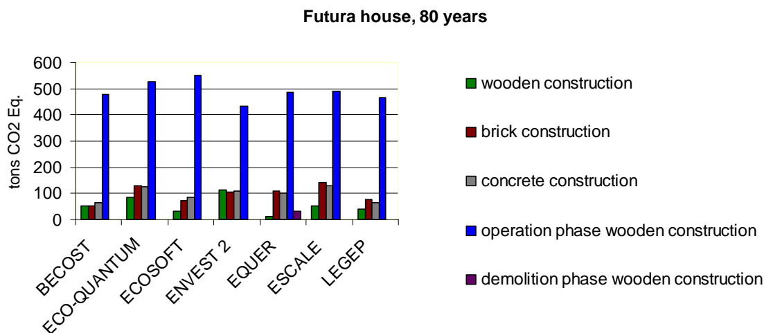
Fig. 4: Predicted global warming potential for the FUTURA house when constructed from different materials. Explanation of the legend
