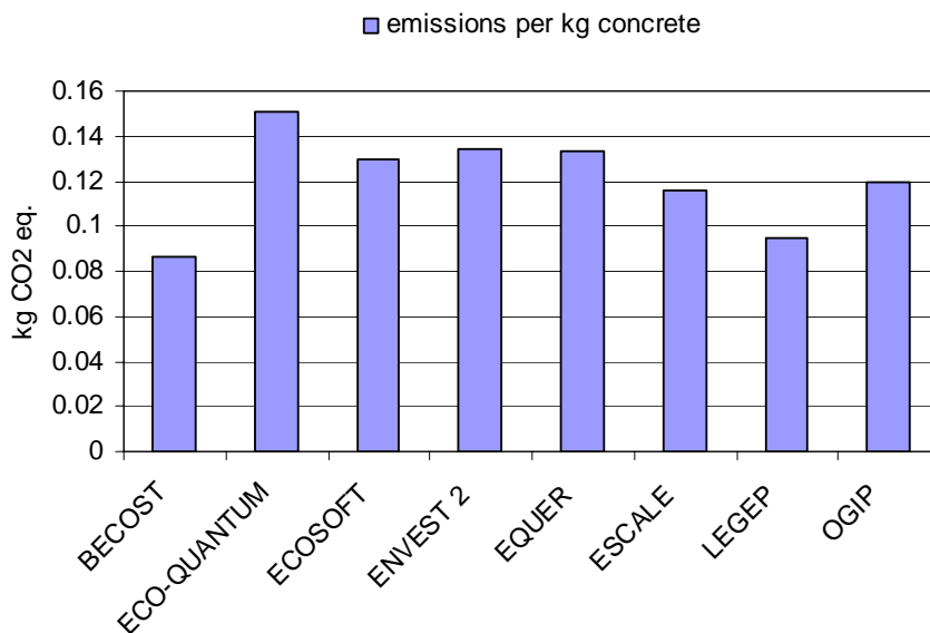
Fig. 1 Predicted Greenhouse gas emissions over 50 years from 1 kg of concrete
